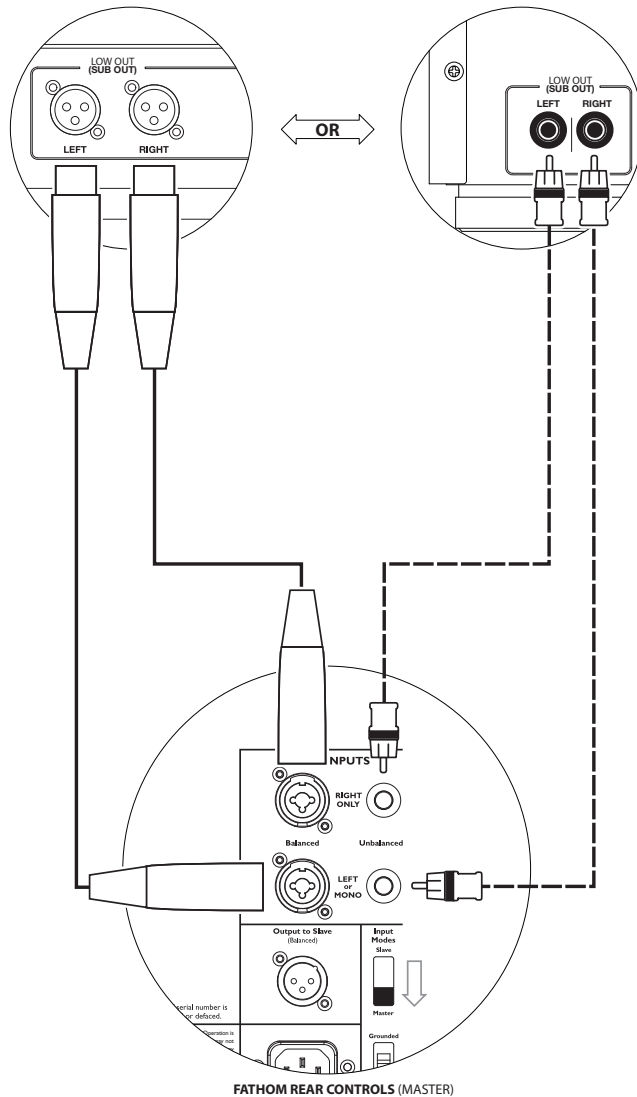
FATHOM REAR CONTROLS (MASTER)
