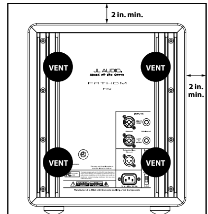
Rear-view of cabinet install:
