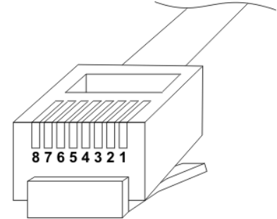
RJ 45 connector
